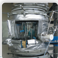
Exposure chamber
